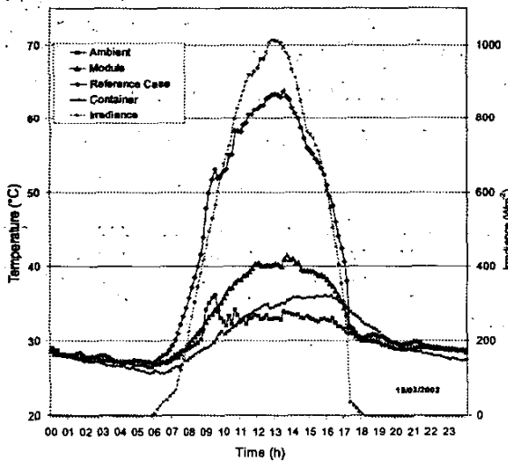
Fig. 5. Temperature measurements of All-in-one-system during a clear day: lower module temperature ("Module") and water temperature in upper part of the container ("Container"), in comparison to a standard module ("Reference Case") and ambient temperature ("Ambient").
