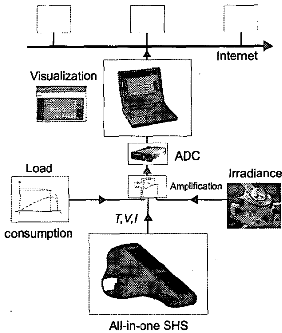
Fig. 4. Configuration of the measurement system for the All-in-one SHS.
