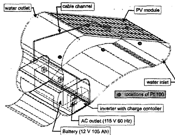
Fig. 1. Structure and components of the all-in-one SHS.
