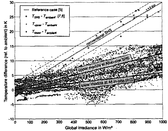
Fig. 6. Measured temperature differences between module and ambient in comparison to the reference case (standard SHS) plotted as a function of irradiance.
