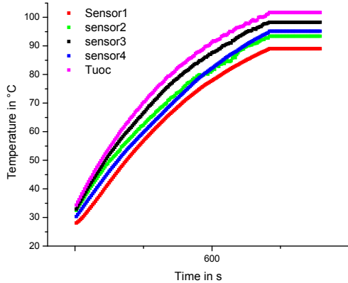
Fig. 3. Heat-up characteristics of a c-Si module in a steady state sun simulator without ventilation at an irradiance of 875 W/m 2 , the type of sensors are listed in Table 5.
